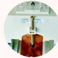
Busbar Support Mounting
