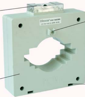
Built In Hinged Sealable Terminal Cover (Metallic sealable screw for option)
